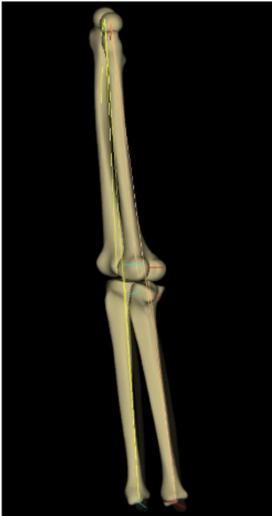
Non-diagnostic image
